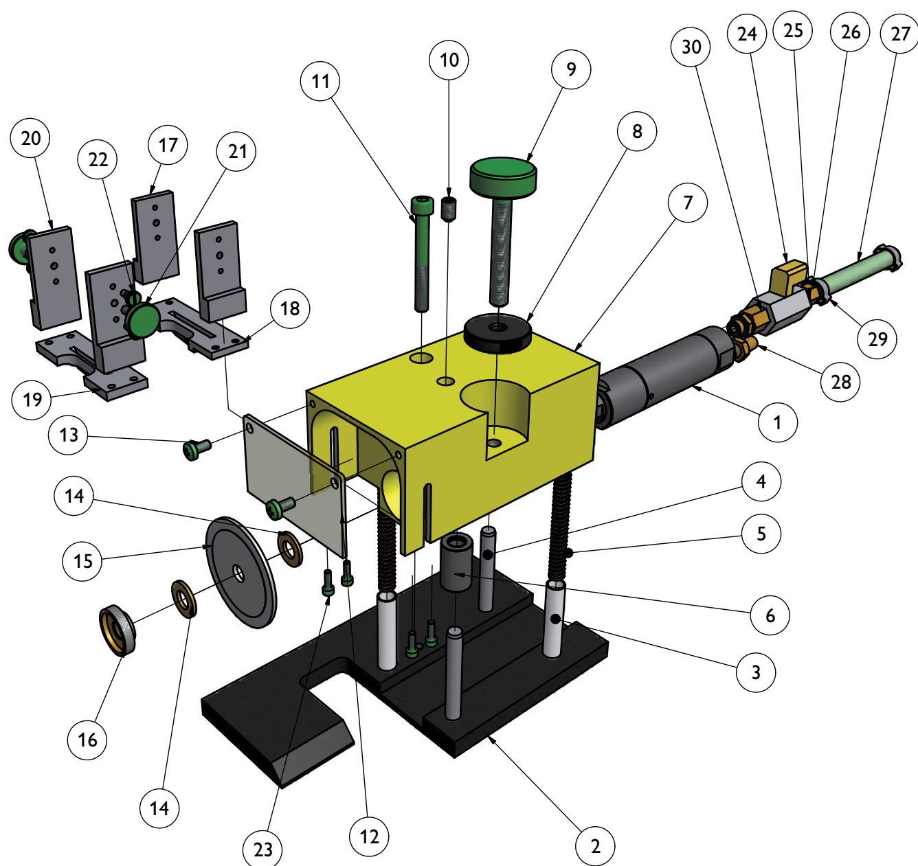
Fig. 3: Exploded drawing
